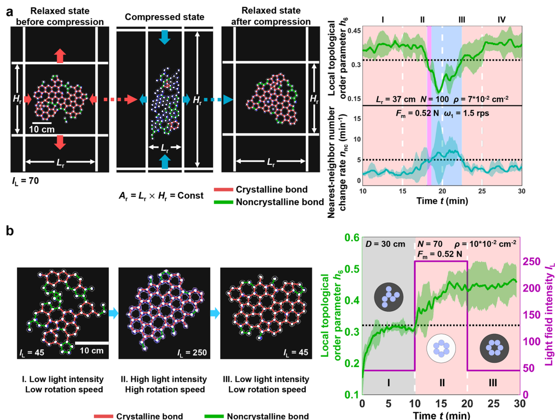
Fig. 6 | Environmental responsiveness of Robo-Matter. a Adaptivity of Robo-Matter in response to external stimuli. Left panels show the snapshots of a reversible active crystal to disordered gas-like phase transition induced by an isovolumetric compression and decompression cycle (Supplementary Movie 2). The right panel shows the evolution of h_6 and the nearest-neighbor number change rate n_{nc} during the process. The stages I, II, III, and IV, respectively corresponds to the relaxed state before compression, the compression process, the decompression process, and the relaxed state after compression. b Structural self-optimization of Robo-Matter in a rapidly changing environmental field. Left panels show the snapshots of a rapid re-organization and self-optimization of an active glass-like
